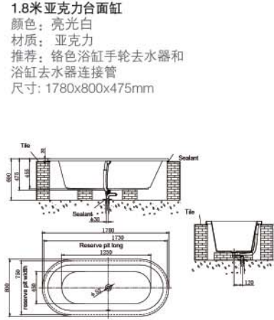
NB25803W 1.8m Acrylic Drop-in Bathtub Color : White Material : Acrylic Recommended Parts : Chromium-color bathtub hand-wheel drainer and connecting pipe of bathtub drainer. Size : 1780x800x475mm 1.8米亚克力台面缸 颜色：亮光白 材质：亚克力 推荐：铬色浴缸手轮去水器和 浴缸去水器连接管 尺寸：1780x800x475mm
